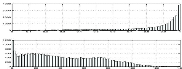
Figure 3: Distribution of a) \Gamma(\omega, t) , b) \epsilon(\omega, t)/f for signal of Figure 2
