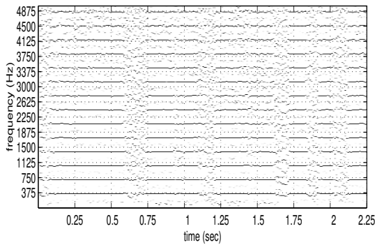
Figure 1: 1 - \Gamma(\omega, t) computed on a) original signal, b) pre-processed signal. Darker values indicate \Gamma(\omega, t) close to 1. Signal : Tibetan female singing voice ( \bar{f}_0(t) =345 Hz, LPC order 40, Blackman-Harris-3 window, 20ms)
