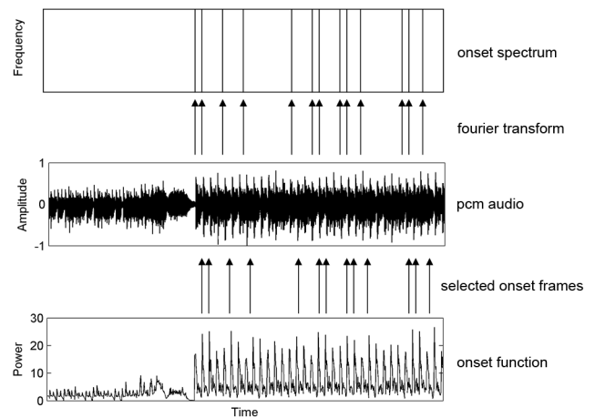
Figure 2: The onset detection function is used to select those time domain windows, which have to be transformed to the frequency domain. The resulting spectral frames are so-called "event vectors".
