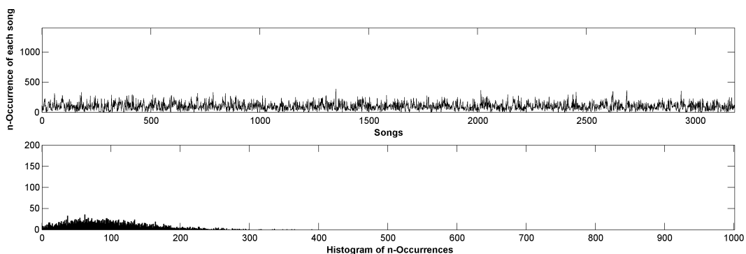
Figure 4: Visualization of the 100-Occurrences of the histogram intersection distance measure (upper plot) and the corresponding histogram. Obviously the distribution is quite different from the distribution in figure 3. Most notably, there are no songs that have an extreme 100-Occurrence value (upper plot), which implies that there are no hubs.
