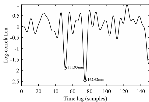
Figure 5: The log-correlation of an electric guitar plucked on the open 4th string at 100 mm from the bridge with a pickup located at 159 mm from the bridge.
