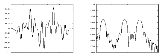
Figure 7. FIR filter extracted from a 3-sine 2D filter.
