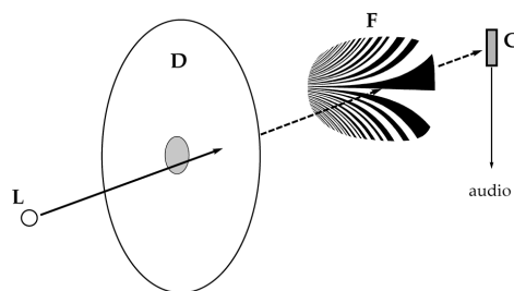
Figure 1. The photosonic optical instrument.
